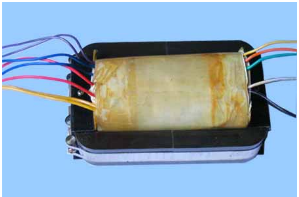
C-Core Power Transformer Used For Elevator Control
